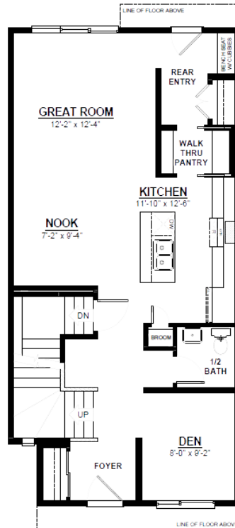
MAIN FLOOR 807 Sq. Ft.
