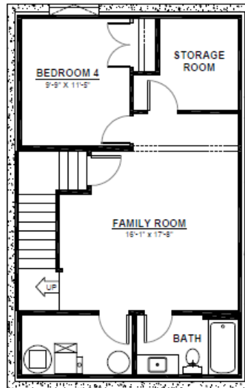
BASEMENT 547 SQ.FT (8 FT. FOUNDATION)
