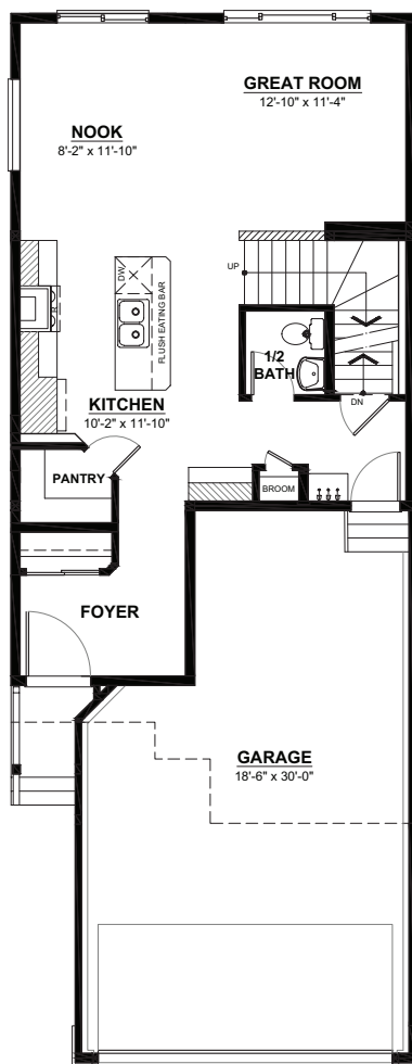
MAIN FLOOR 689sq.ft. (9FT. CEILINGS)
