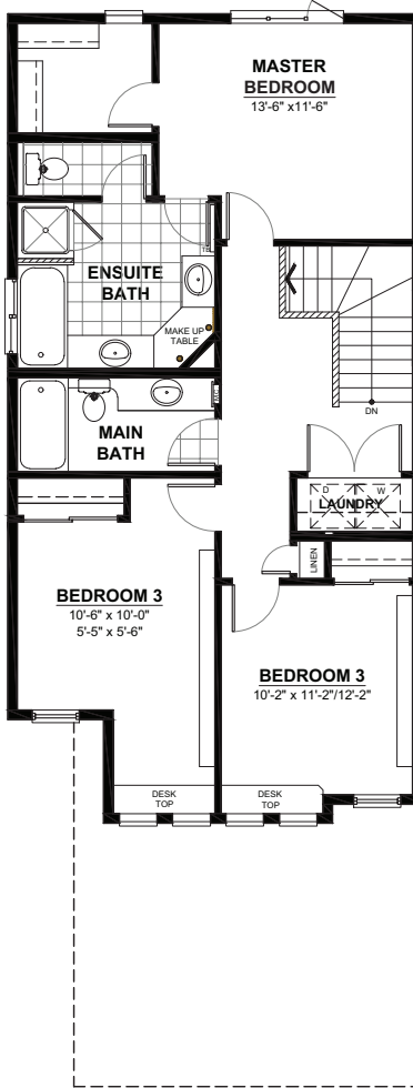
2ND FLOOR 870sq.ft. (8FT. CEILINGS)
